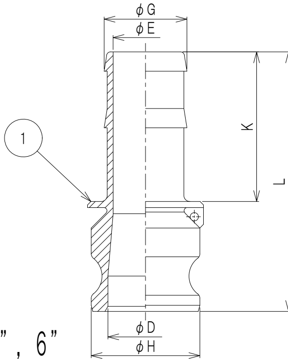
6 3 3 - E S S T DIMENSION TABLE BY SIZES (UNIT:mm)
